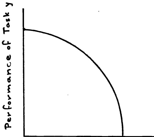
Performance of Task x [from Navon & Gopher (1979)]
